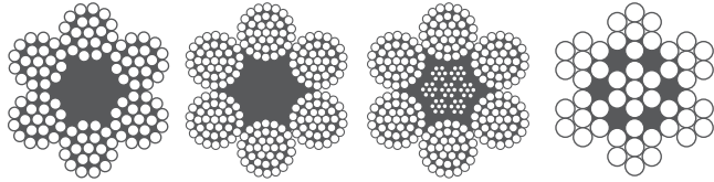
6 x 19 Fibre Core 6 x 37 Fibre Core 6 x 37 Wire Core 7 x 7 Wire Core
